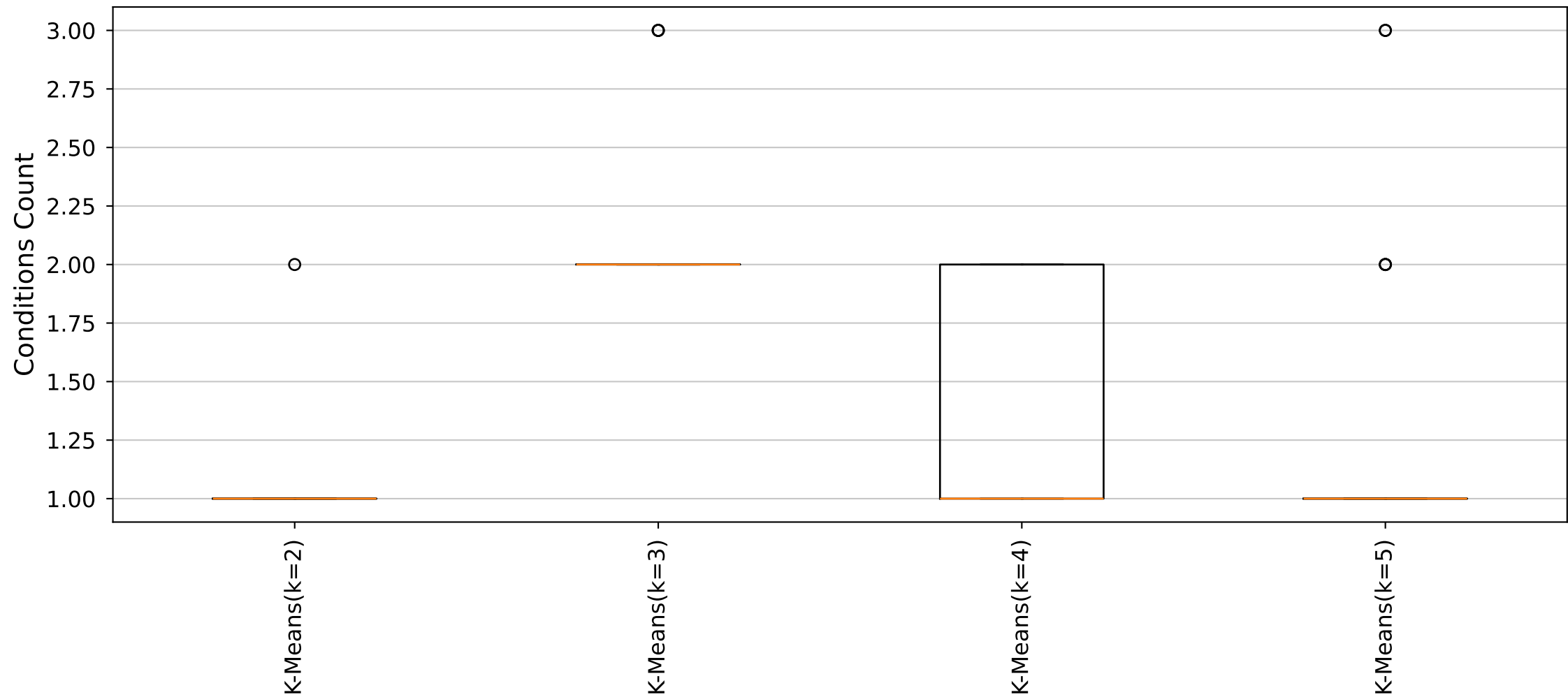
YARA Rules Conditions Count Distribution (Cluster40_Size5 dataset)
